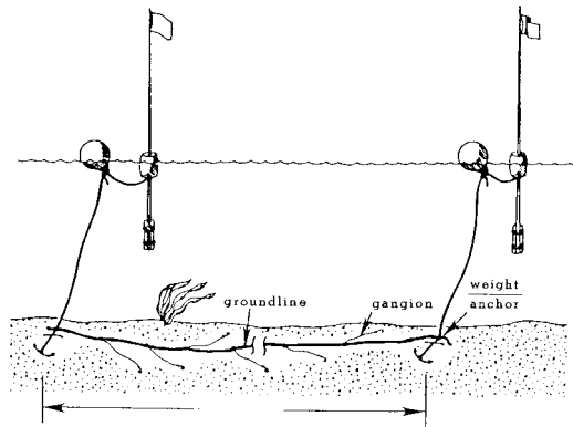
Halibut longline gear
